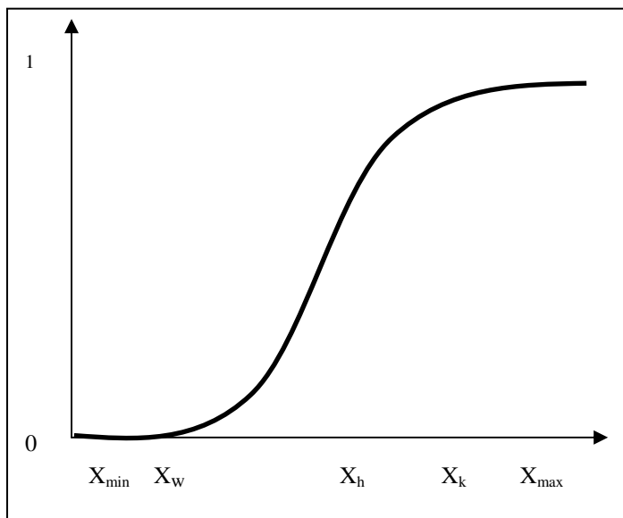
Figure 3. Sigmoid curve / function
